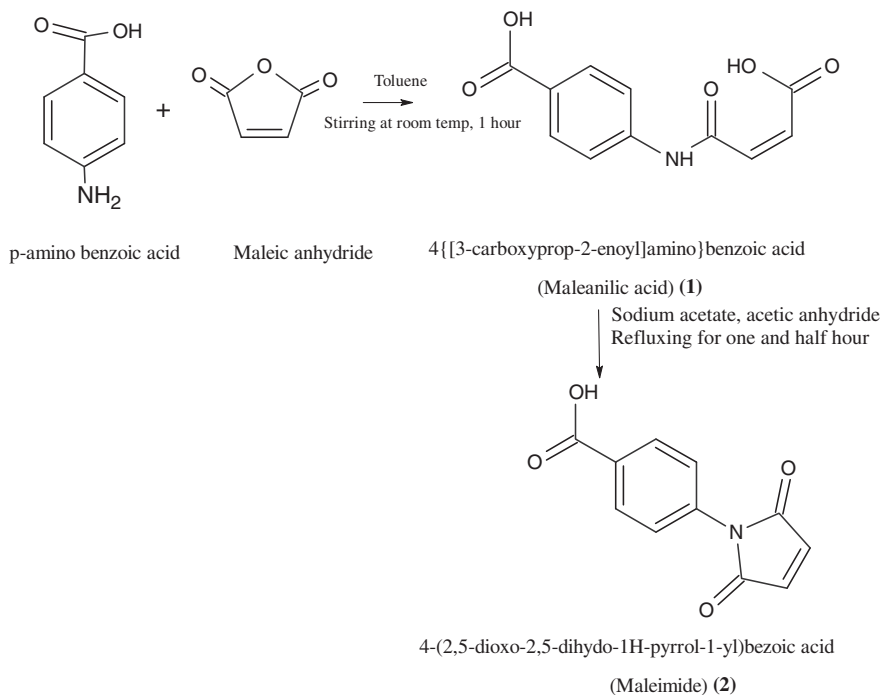
Figure 1. Schematic diagram describing the steps in the synthesis of maleimide from p -aminobenzoic acid.
