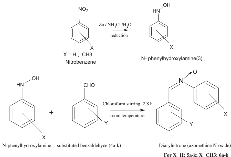
Figure 2. Schematic diagram describing the synthesis of differently substituted nitrones.
