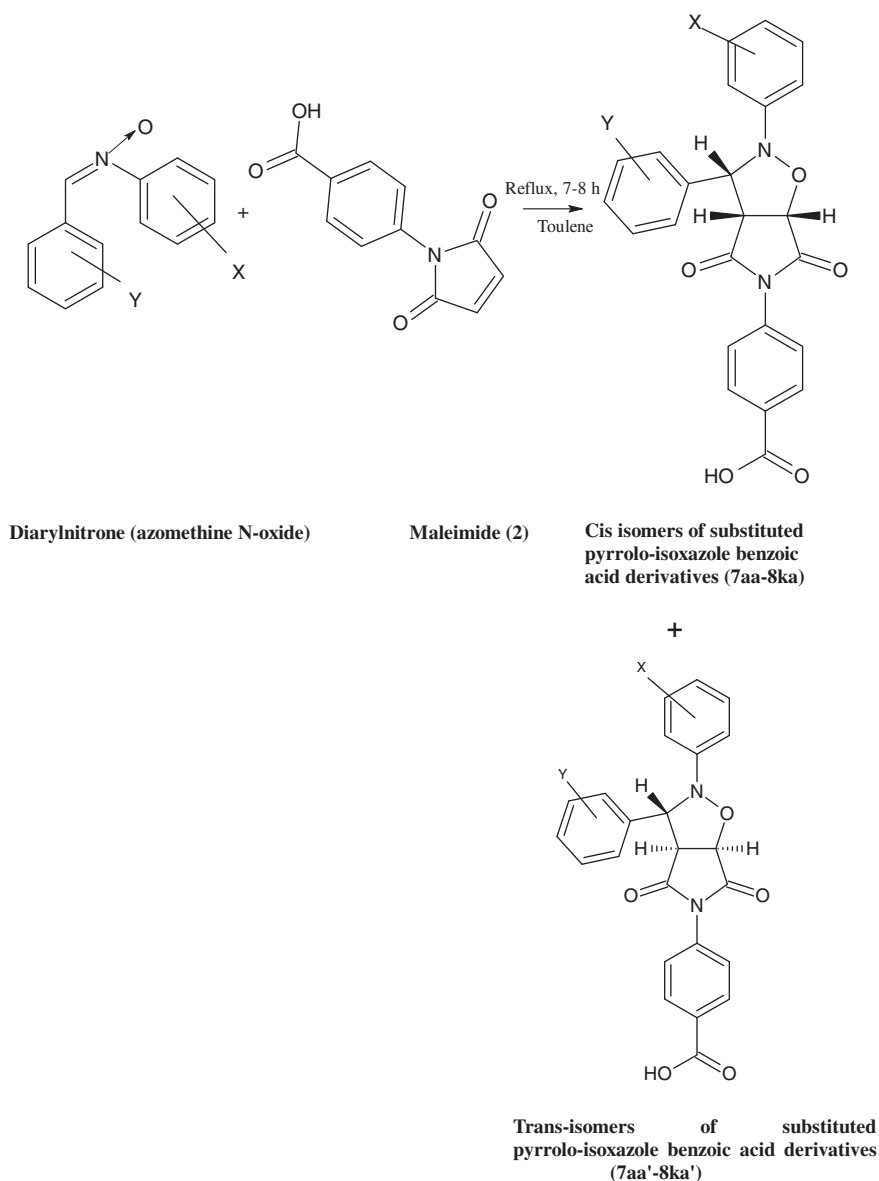
Figure 3. Schematic diagram describing the steps in the synthesis of substituted cis - and trans -isomers from differently substituted diaryl nitrones and maleimide.
